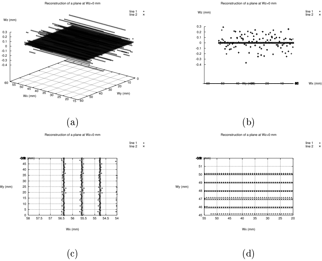
Figure A.3: Reconstruction of a plane at Wz=0 .
