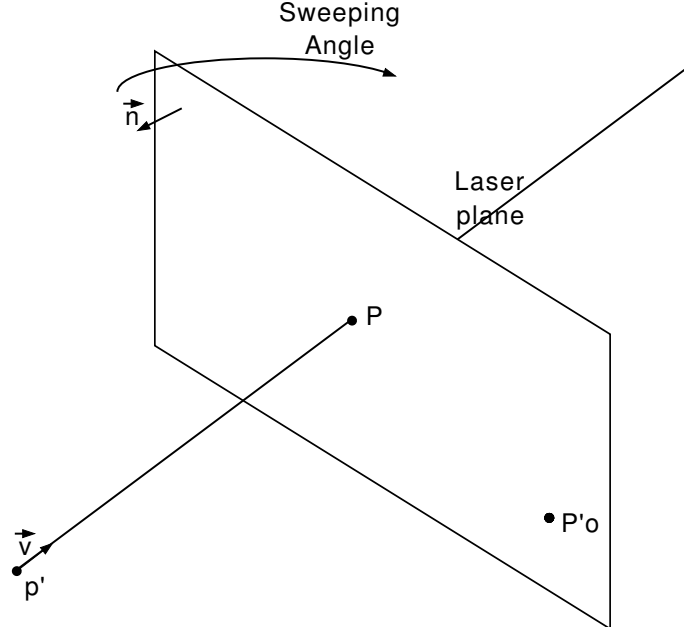
Figure 2.3: 3D reconstruction by triangulation using a laser plane and a camera.
