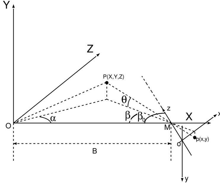
Figure 2.13: Yu et al. digitiser geometric parameters.
