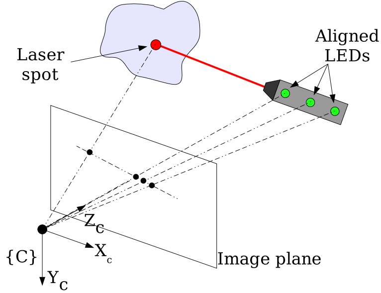
Figure 2.9: Low cost wand scanner.
